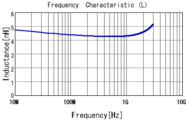
LQG15WZ4N3B02 L
