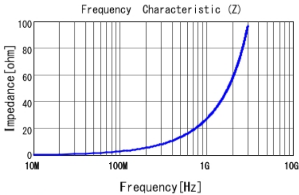
LQG15WZ4N3B02 |Z|
