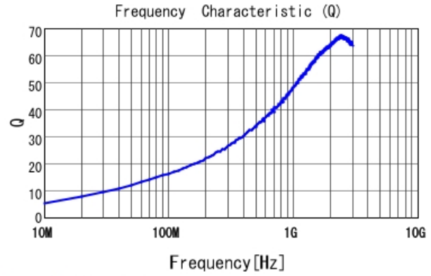
LQG15WZ4N7B02 Q
