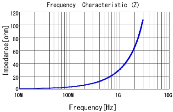
LQG15WZ4N7B02 |Z|
