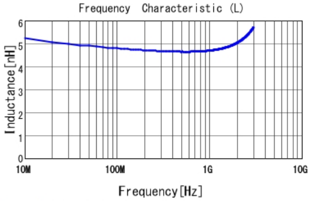
LQG15WZ4N7B02 L
