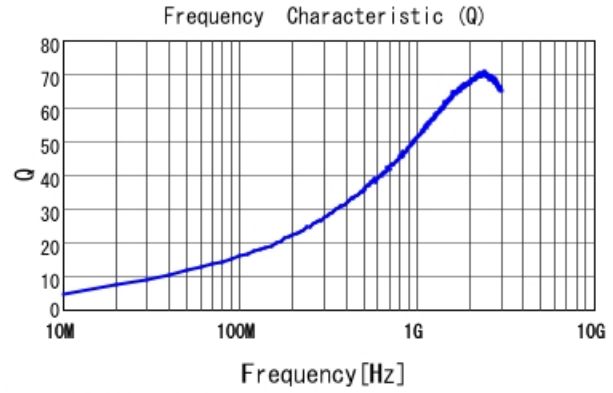
LQG15WZ5N1B02 Q
