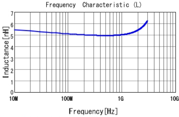
LQG15WZ5N1B02 L
