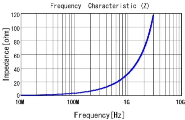
LQG15WZ5N1B02 |Z|
