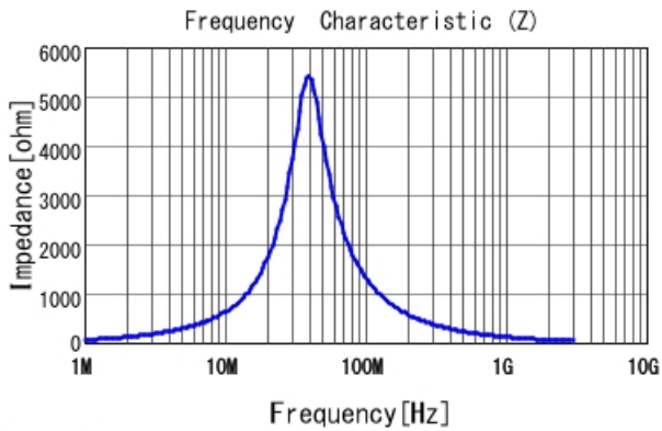
LQM18DH100M70 |Z|
