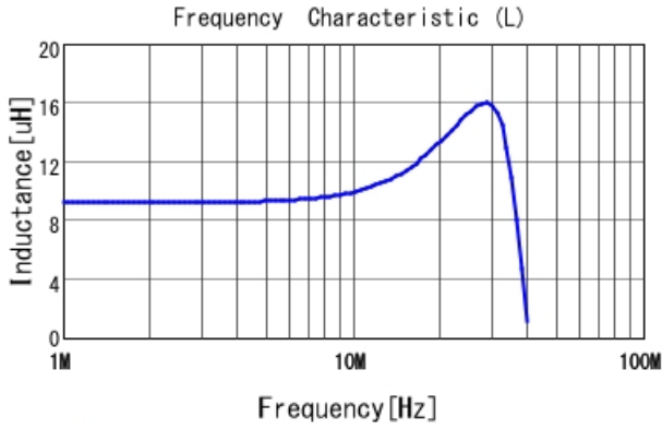
LQM18DH100M70 L
