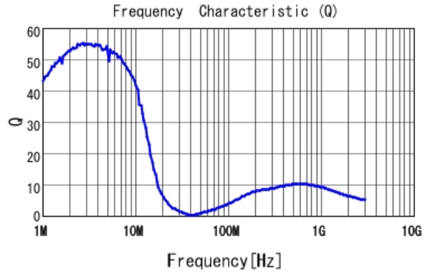
LQM18DH100M70 Q
