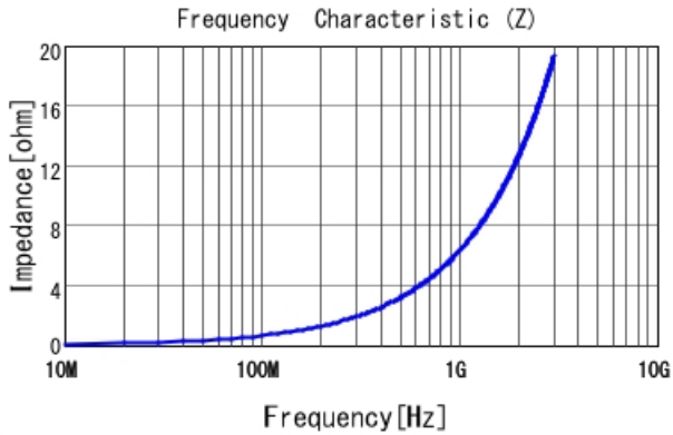
LQW04AN1N1D00 |Z|
