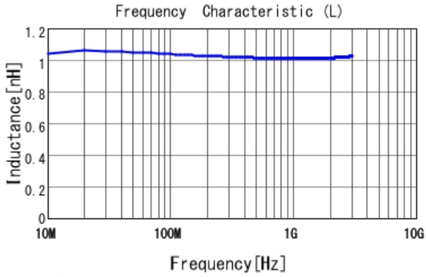
LQW04AN1N1D00 L
