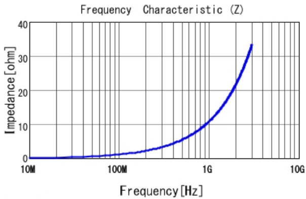
LQW04AN1N8D00 |Z|
