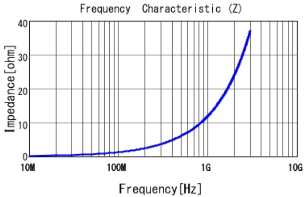
LQW04AN1N9D00 |Z|
