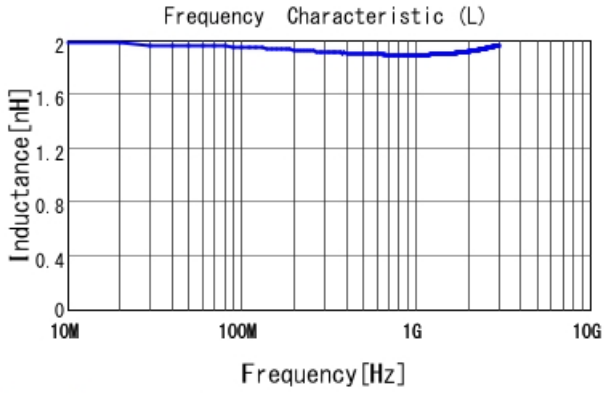
LQW04AN1N9D00 L
