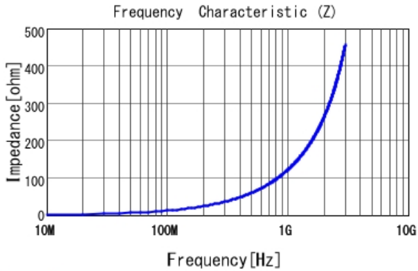
LQW04AN20NJ00 |Z|
