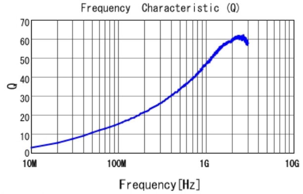
LQW04AN20NJ00 Q
