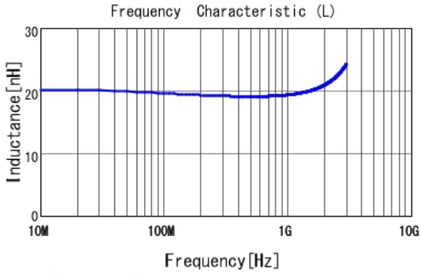
LQW04AN20NJ00 L
