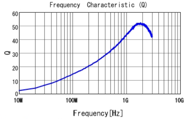
LQW04AN27NJ00 Q
