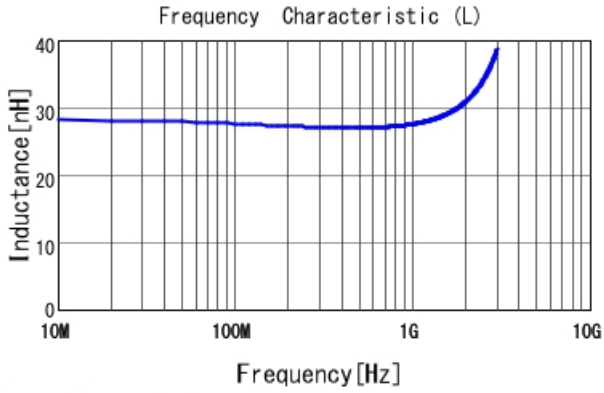
LQW04AN27NJ00 L
