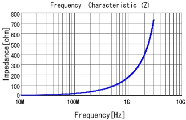
LQW04AN27NJ00 |Z|
