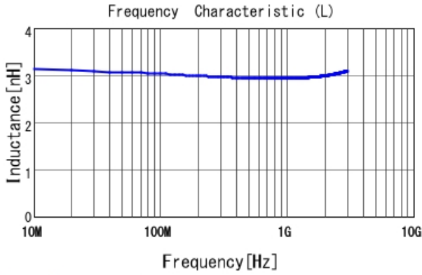
LQW04AN2N9D00 L
