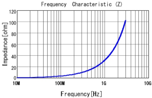
LQW04AN5N0D00 |Z|
