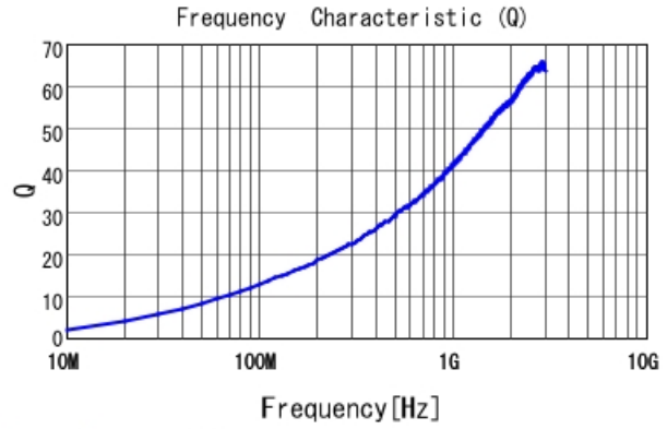
LQW04AN5N0D00 Q
