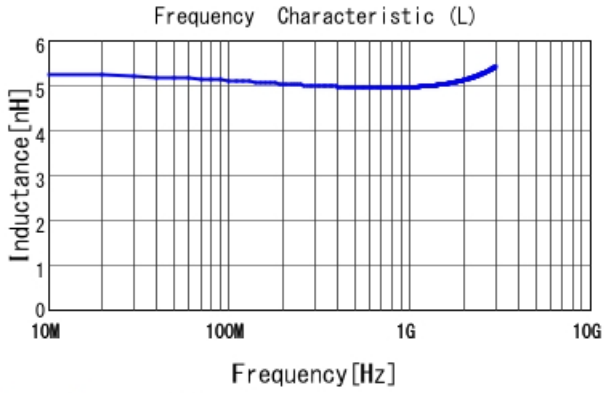
LQW04AN5N0D00 L
