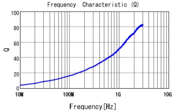
LQW04AN5N1D00 Q
