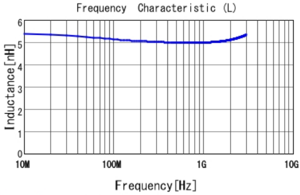
LQW04AN5N1D00 L
