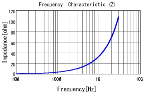
LQW04AN5N3D00 |Z|
