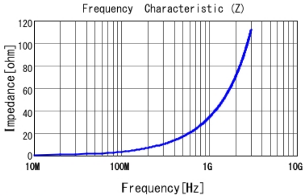
LQW04AN5N5D00 |Z|
