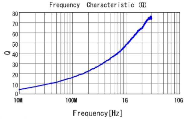
LQW04AN5N5D00 Q
