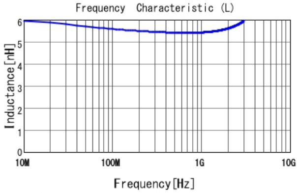
LQW04AN5N5D00 L
