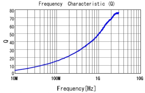
LQW04AN6N8D00 Q
