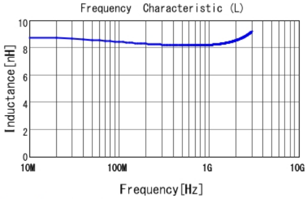
LQW04AN8N2D00 L
