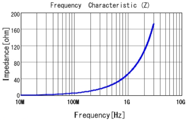
LQW04AN8N2D00 |Z|
