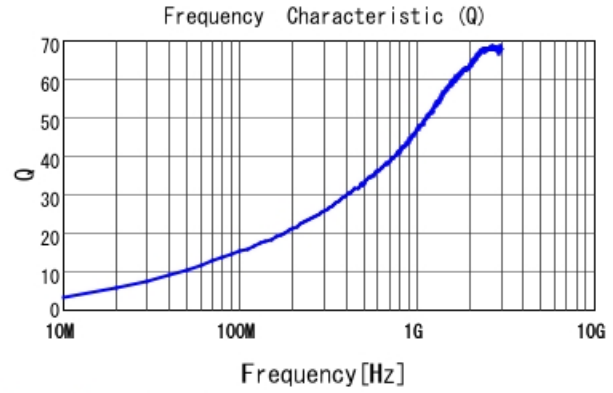
LQW04AN8N2D00 Q
