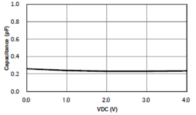
Voltage—Capacitance Characteristic
