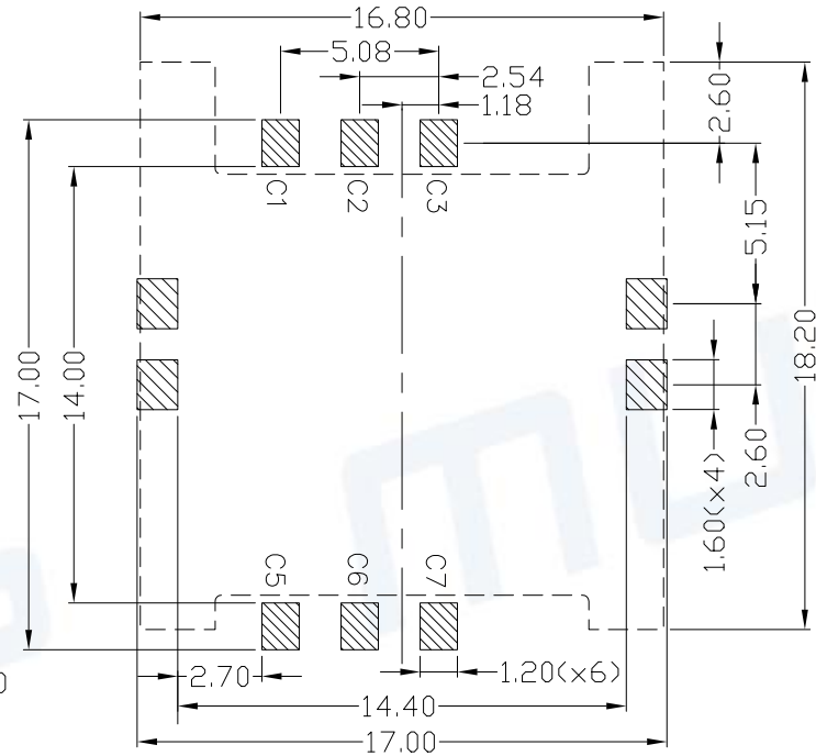
RECOMMENDED P.C.B LAYOUT COMPONENT SIDE(TOLERANCE ±0.05)
