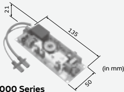
MPL3000 Series
