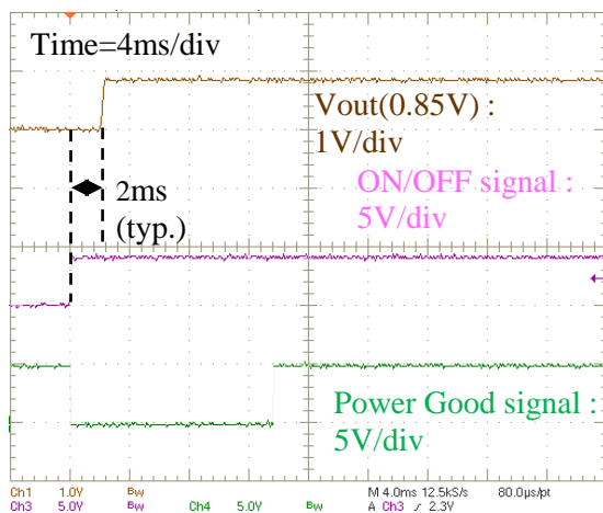
On/Off Enable Delay (Vin=5.0V, Vout=0.85V, Iout=0A, Cloud=110uF)
