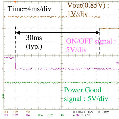
On/Off Enable Delay (Vin=5.0V, Vout=0.85V, Iout=0A, Cloud=110uF)
