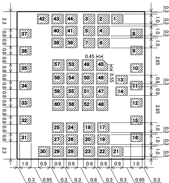
< Bottom View >
