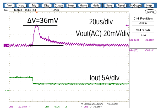
Step Load Transient Response (Vin=12V, Vout=1.0V, Cload=400uF, Iout=6A to 3A, 2.5A/us)
