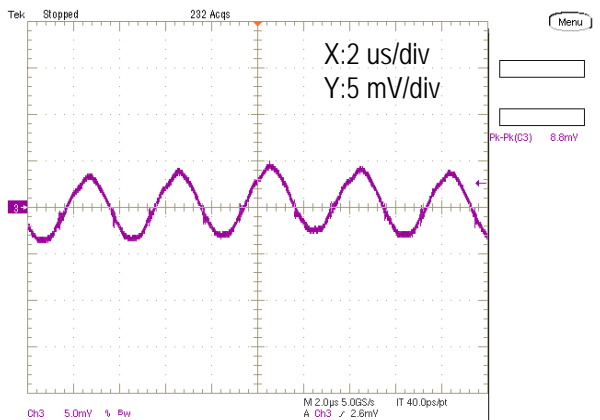
Output Ripple and Noise (Vin=5.0V, Vout=1.8V, Iout=6A, Load=400uF, ScopeBW=20MHz)
