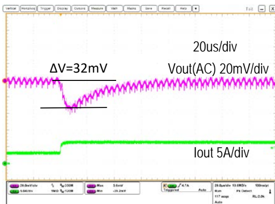
Step Load Transient Response (Vin=5.0V, Vout=1.8V, Load=400uF, Iout=3A to 6A, 2.5A/us)
