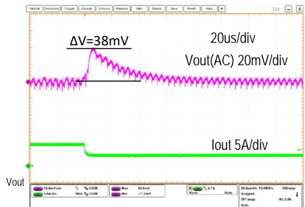
Step Load Transient Response (Vin=5.0V, Vout=1.8V, Load=400uF, Iout=6A to 3A, 2.5A/us)
