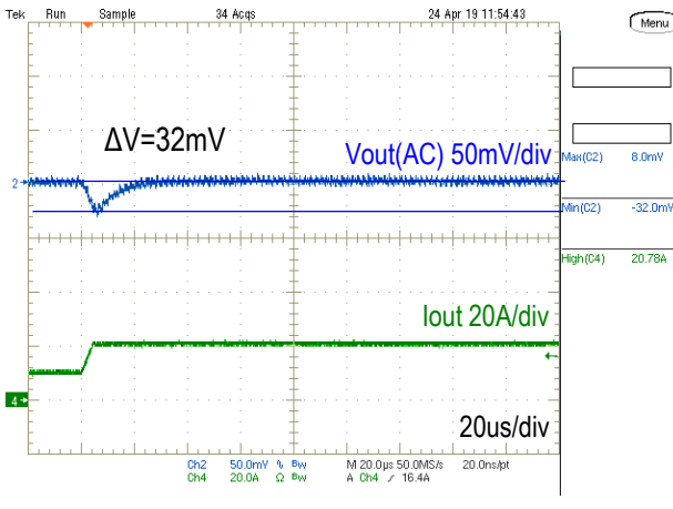
Step Load Transient Response (Vin=5.0V, Vout=1.0V, Cload=660uF, Iout=10A to 20A, 1.0A/us) Trace 2=Vout(AC), 50mV/div, Trace 4=Iout, 20A/div, 20us/div
