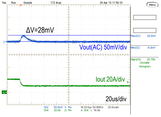
Step Load Transient Response (Vin=5.0V, Vout=1.0V, Cload=660uF, Iout=20 to 10A, 1.0A/us) Trace 2=Vout(AC), 50mV/div, Trace 4=Iout, 20A/div, 20us/div
