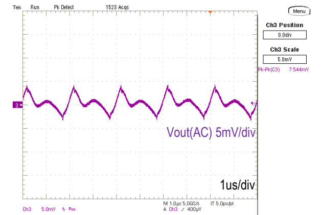
Output Ripple and Noise (Vin=5.0V, Vout=1.0V, Iout=20A, Cload=660uF, Scope BW=20MHz, 5mV/div, 1us/div)
