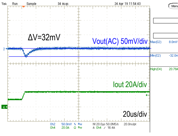
Step Load Transient Response (Vin=5.0V, Vout=1.0V, Cload=660uF, Iout=10A to 20A, 1.0A/us) Trace 2=Vout(AC), 50mV/div, Trace 4=Iout, 20A/div, 20us/div
