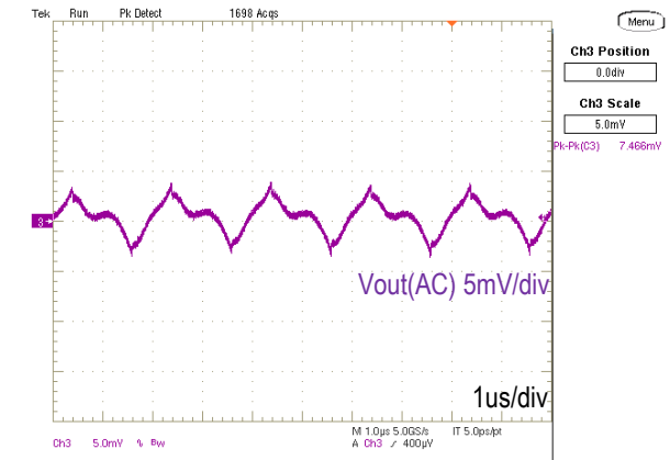
Output Ripple and Noise (Vin=5.0V, Vout=1.8V, Iout=20A, Cload=660uF, Scope BW=20MHz, 5mV/div, 1us/div)
