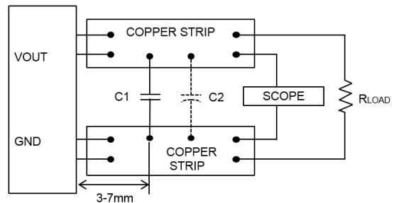
C1=220uF x 3 CERAMIC C2=OPEN
