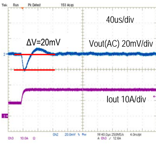
Step Load Transient Response (Vin=12V, Vout=0.7V, Load=660uF, Iout=8A to 16A 2.4A/us)
