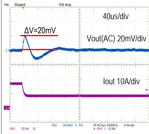
Step Load Transient Response (Vin=12V, Vout=0.7V, Load=660uF, Iout=16 to 8A 2.4A/us)
