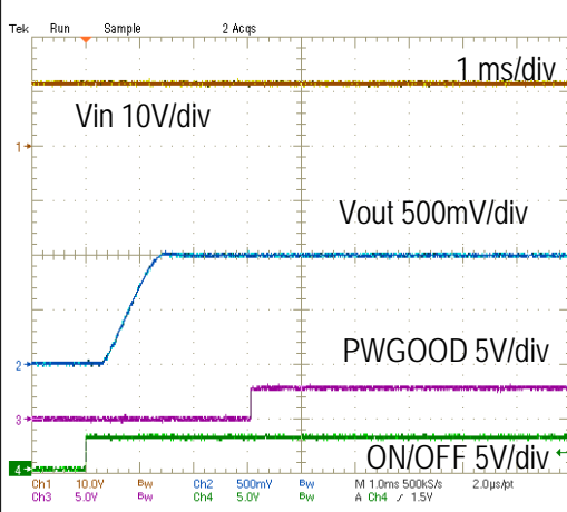
On/Off Enable Delay (Vin=12V, Vout=1.0V, Iout=16A, Cload=660uF)
