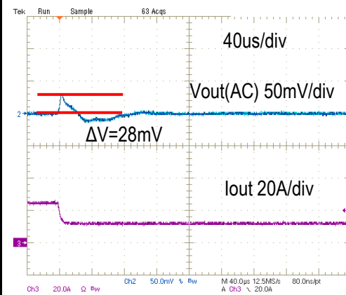
Step Load Transient Response (Vin=12V, Vout=1.0V, Cload=660uF, Iout=24A to 12A, 2.4A/us)
