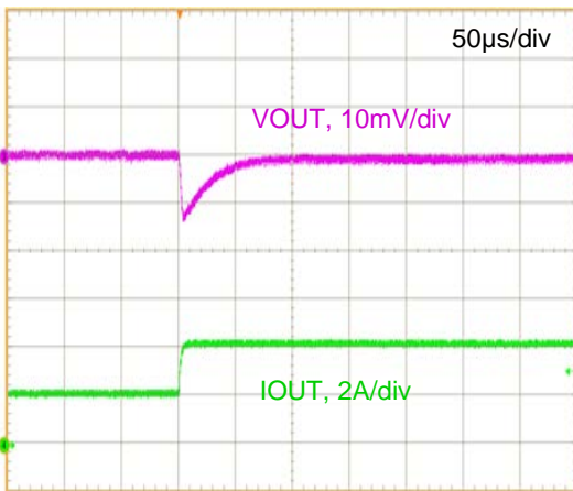
Figure 27. Step Load Transient Response (VIN=12V, VOUT=0.7V, COUT=200μF, IOUT=2 to 4A, 1.0A/μs)
