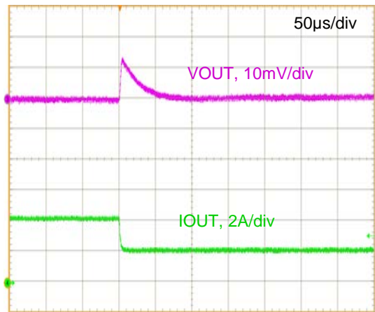
Figure 28. Step Load Transient Response (VIN=12V, VOUT=0.7V, COUT=200μF, IOUT=4 to 2A, 1.0A/μs)
