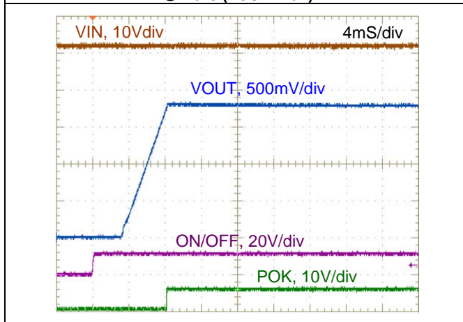
Figure 13. On/Off Enable wave form @+25°C (VIN=12V, VOUT=1.8V, IOUT=4A)
