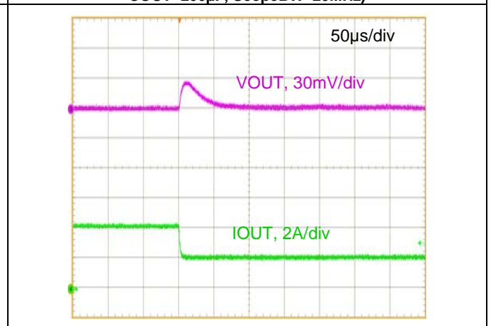
Figure 16. Step Load Transient Response (VIN=12V, VOUT=1.8V, COUT=200μF, IOUT=4 to 2A, 1.0A/μs)
