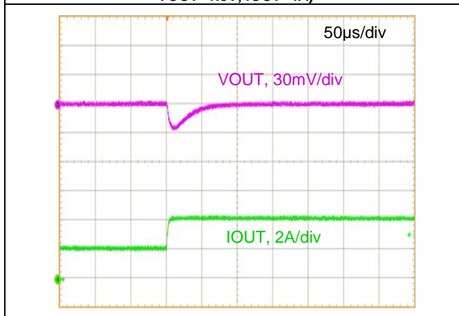
Figure 15. Step Load Transient Response (VIN=12V, VOUT=1.8V, COUT=200μF, IOUT=2 to 4A, 1.0A/μs)
