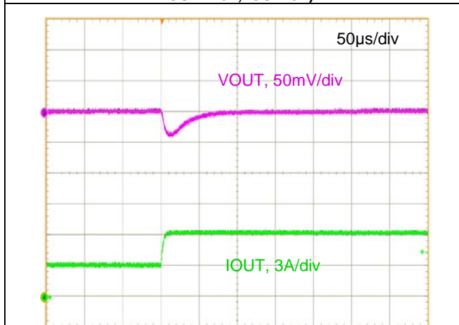
Figure 15. Step Load Transient Response (VIN=12V, VOUT=1.8V, COUT=200µF, IOUT=3 to 6A, 1.0A/µs)
