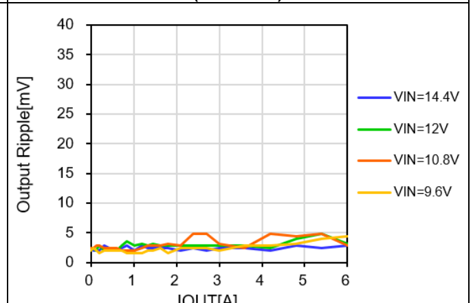
Figure 14. Output Ripple and Noise @+25°C (VOUT=1.8V, COUT=200µF, ScopeBW=20MHz)
