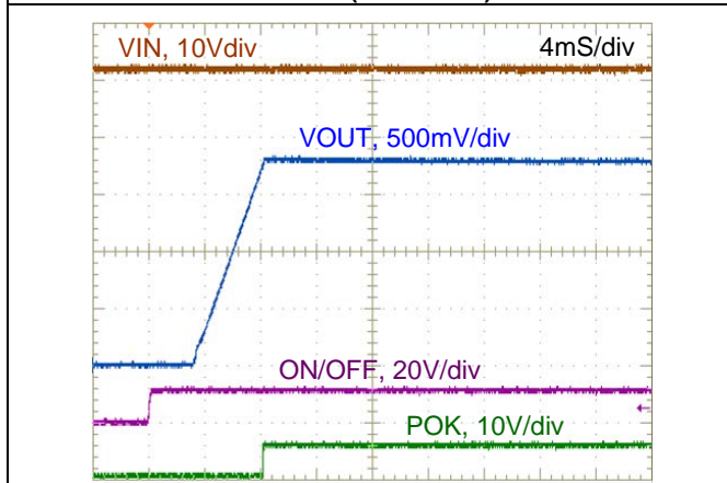
Figure 13. On/Off Enable wave form @+25°C (VIN=12V, VOUT=1.8V, IOUT=6A)
