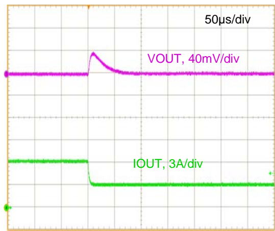
Figure 22. Step Load Transient Response (VIN=12V, VOUT=1.2V, COUT=200μF, IOUT=6 to 3A, 1.0A/μs)
