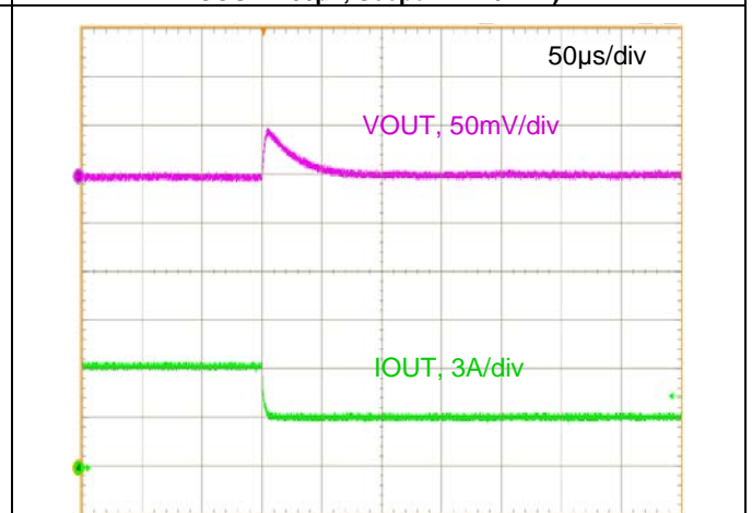
Figure 16. Step Load Transient Response (VIN=12V, VOUT=1.8V, COUT=200µF, IOUT=6 to 3A, 1.0A/µs)
