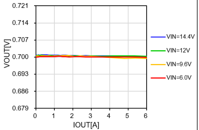
Figure 24. VOUT vs. Load Current and Line Voltage @+25°C (VOUT= 0.7V)
