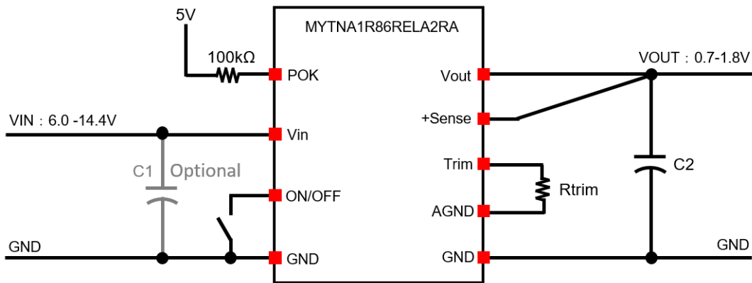
Figure 33. Application Schematic
