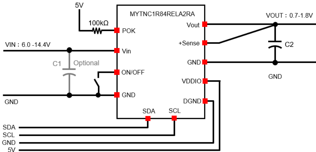
Figure 39. Application Schematic
