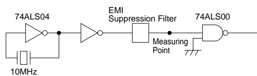
Measuring Circuit
