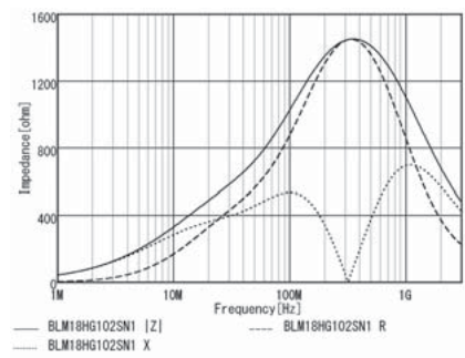
BLM18HG102SN1
