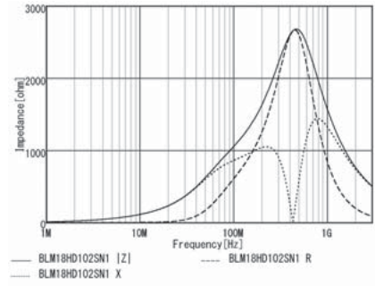
BLM18HD102SN1
