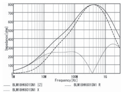
BLM18HK601SN1
