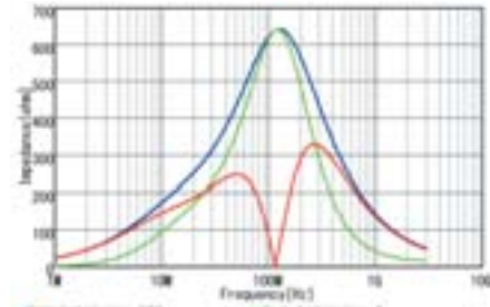
BLM18KG601SZ1/BLM18KG601SH1
