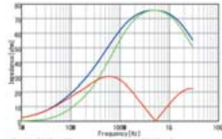
BLM18KG700TZ1/BLM18KG700TH1
