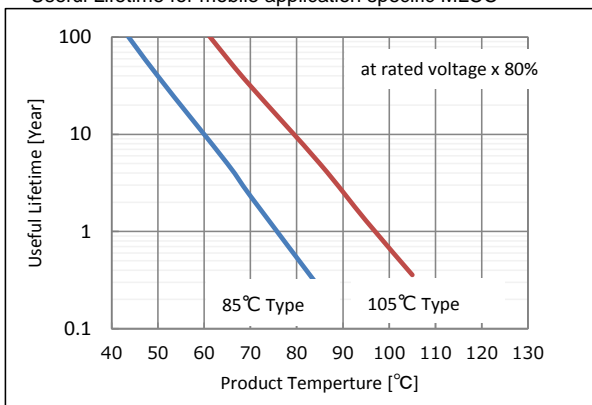
Useful Lifetime for mobile application specific MLCC
