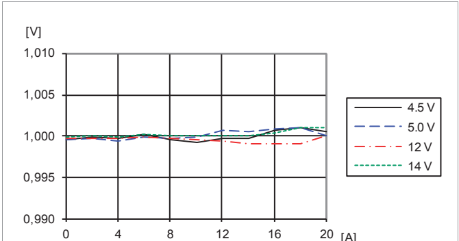
Load regulation, V_O=1.0\text{ V}
