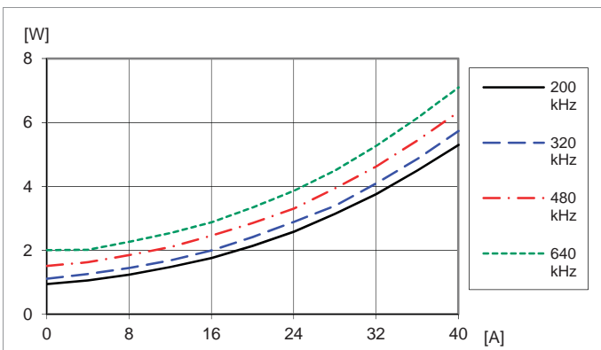
Dissipated power vs. load current and switch frequency at T_{P1} = +25\text{ }^\circ\text{C} , V_i = 12\text{ V} , V_0 = 1.0\text{ V} , C_0 = 470\text{ }\mu\text{F}/10\text{ m}\Omega Default configuration except changed frequency
