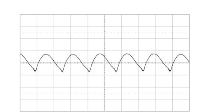
Output Ripple & Noise, V_O = 1.0\text{ V}
