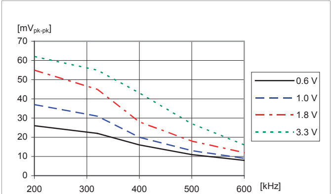
Output Ripple vs. Frequency
