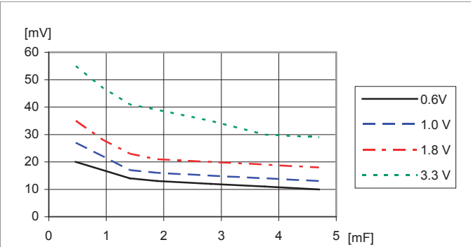
Output Ripple vs. External Capacitance
