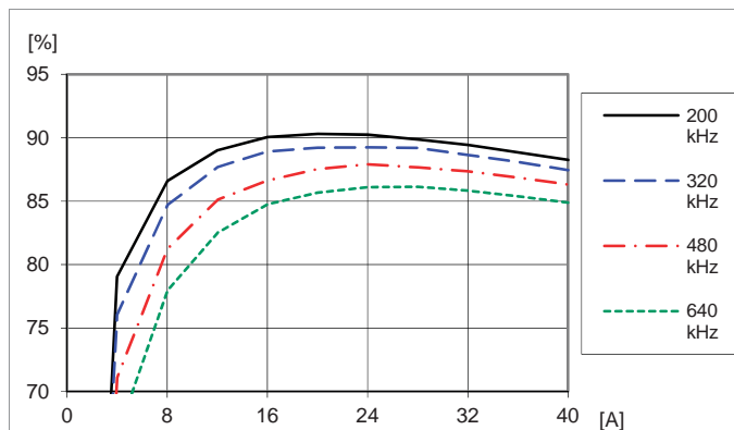
Efficiency vs. load current and switch frequency at T_{P1} = +25\text{ }^\circ\text{C} , V_i = 12\text{ V} , V_0 = 1.0\text{ V} , C_0 = 470\text{ }\mu\text{F}/10\text{ m}\Omega Default configuration except changed frequency
