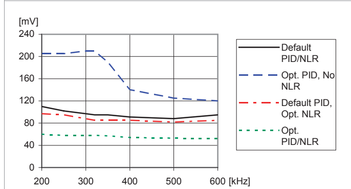
Load transient peak voltage deviation vs. frequency. Step-change (5-15-5 A). T_{P1} = +25 °C, V_I = 12 V, V_O = 1.0 V, C_O = 470 \mu F/10 m \Omega
