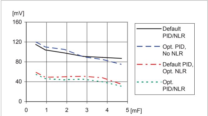
Load transient peak voltage deviation vs. external capacitance. Step-change (5-15-5 A). Parallel coupling of capacitors with 470 \mu F/10 m \Omega , T_{P1} = +25 ^{\circ} C, V_I = 12 V, V_O = 3.3 V, f_{sw} = 320 kHz, di/dt = 2 A/ \mu s
