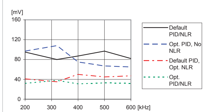
Load transient peak voltage deviation vs. frequency. Step-change (5-15-5 A). T_{P1} = +25 ^{\circ} C, V_I = 12 V, V_O = 1.0 V, C_O = 470 \mu F/10 m \Omega
