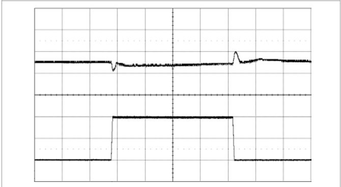
Output voltage response to load current step-change (5-15-5 A) at: T_{P1} = +25 °C, V_I = 12 V, V_O = 1.0 V, di/dt = 2 A/ \mu s, f_{sw} = 320 kHz, C_O = 470 \mu F/10 m \Omega
