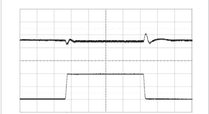
Output voltage response to load current step-change (5-15-5 A) at: T_{P1} = +25 ^{\circ} C, V_I = 12 V, V_O = 1.0 V, di/dt = 2 A/ \mu s, f_{sw} = 320 kHz, C_O = 470 \mu F/10 m \Omega Top trace: output voltage (200 mV/div.). Bottom trace: load current (5 A/div.). Time scale: (0.1 ms/div.).
