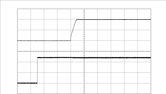
Start-up enabled by connecting V_i at: T_{P1} = +25\text{ }^\circ\text{C} , V_i = 12\text{ V} , V_o = 1.0\text{ V} C_o = 470\text{ }\mu\text{F}/10\text{ m}\Omega , I_o = 50\text{ A} Top trace: output voltage (0.5 V/div.). Bottom trace: input voltage (5 V/div.). Time scale: (20 ms/div.).
