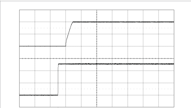
Start-up by enabling CTRL signal at: T_{P1} = +25\text{ }^\circ\text{C} , V_i = 12\text{ V} , V_o = 1.0\text{ V} C_o = 470\text{ }\mu\text{F}/10\text{ m}\Omega , I_o = 50\text{ A} Top trace: output voltage (0.5 V/div.). Bottom trace: CTRL signal (2 V/div.). Time scale: (20 ms/div.).
