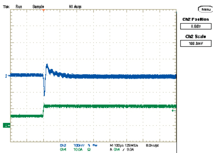
Step Load Transient Response (Vin=12V, Vout=2.5V, Cload=188µF, Iout=6A to 12A) Trace 2=Vout, 100 mV/div, Trace 4=Iout, 10A/div.
