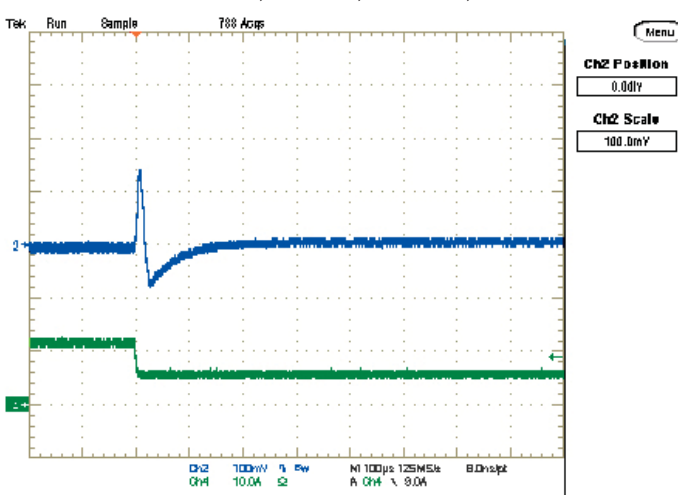
Step Load Transient Response (Vin=11V, Vout=1.2V, Cload=188µF, Iout=12A to 6A) Trace 2=Vout, 100 mV/div, Trace 4=Iout, 10A/div.
