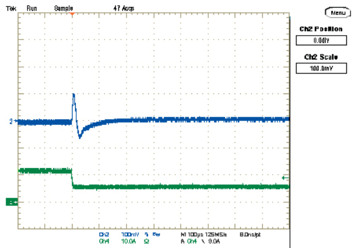
Step Load Transient Response (Vin=7V, Vout=0.69V, Cload=188µF, Iout=12A to 6A) Trace 2=Vout, 100 mV/div, Trace 4=Iout, 10A/div.
