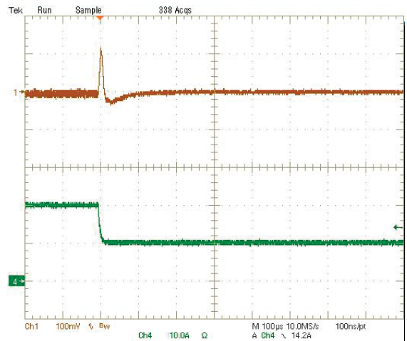
Step Load Transient Response (Vin=12V, Vout=5.0V, Cloud=188µF, Iout=20A to 10A) Trace 1=Vout, 100 mV/div(AC), Trace 4=Iout, 10A/div.
