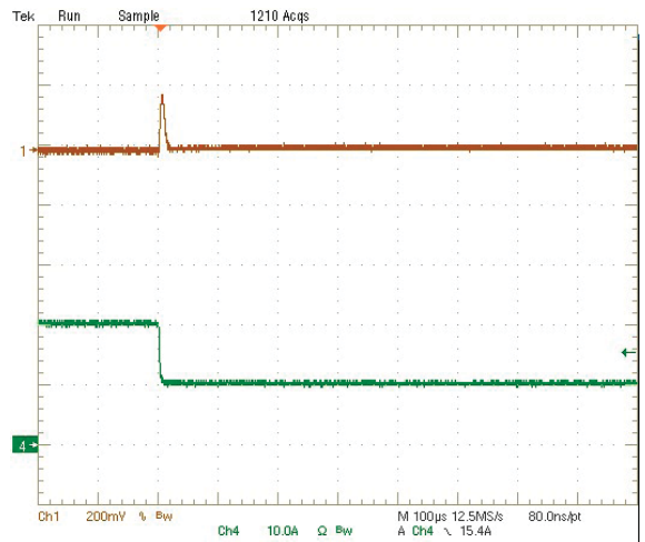
Step Load Transient Response (Vin=5.0V, Vout=3.3V, Cload=94µF, Iout=20A to 10A) Trace 1=Vout, 200 mV/div, Trace 4=Iout, 10A/div.
