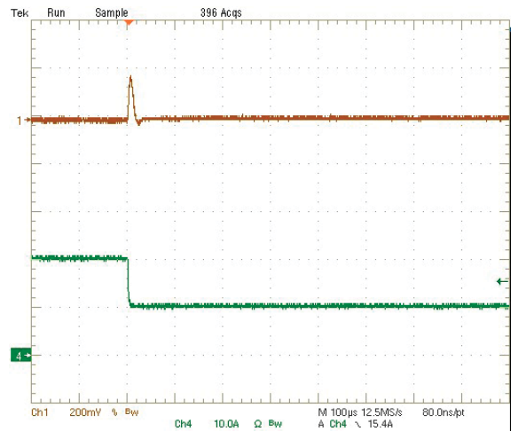
Step Load Transient Response (Vin=5V, Vout=1.2V, Cload=94µF, Iout=20A to 10A) Trace 1=Vout, 200 mV/div, Trace 4=Iout, 10A/div.
