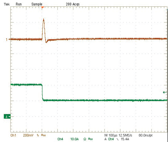
Step Load Transient Response (Vin=5V, Vout=0.6V, Cload=94µF, Iout=20A to 10A) Trace 1=Vout, 200 mV/div, Trace 4=Iout, 10A/div.
