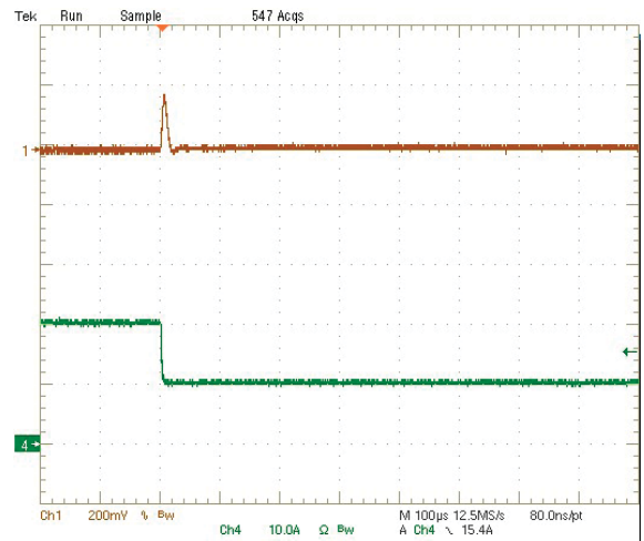
Step Load Transient Response (Vin=5.0V, Vout=2.5V, Cload=94µF, Iout=20A to 10A) Trace 1=Vout, 200 mV/div, Trace 4=Iout, 10A/div.
