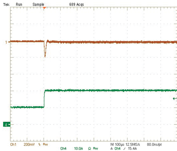
Step Load Transient Response (Vin=5.0V, Vout=1.2V, Cload=94µF, Iout=6A to 12A) Trace 1=Vout, 200 mV/div, Trace 4=Iout, 10A/div.
