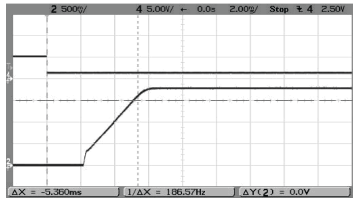
On/Off Enable Startup (V in =5V, V out =1.8V, I out =6A, Cload=0) Trace 4=Enable, Trace 2=V out
