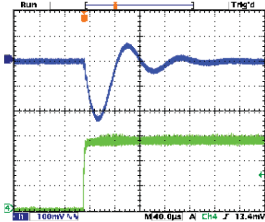
Step Load Transient Response (Vin=5.5V, Vout=3.3V, Load=10x10µF X5R 0805 ceramic, plus 1x470µF, 7mΩ POSCAP, total 570µF, Iout=0A to 1.5A) Top trace=Vout, Bottom trace=Iout
