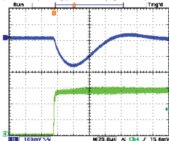
Step Load Transient Response (Vin=12V, Vout=1.8V, Load=10x10µF X5R 0805 ceramic, plus 1x470µF, 7mΩ POSCAP, total 570µF, Iout=1.5A to 0A) Top trace=Vout, Bottom trace=Iout
