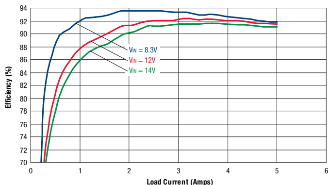
Efficiency vs. Line Voltage and Load Current @ +25°C (V OUT = 3.3V)
