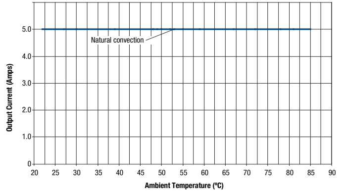
OKY-T/5-W5 Maximum Current Temperature Derating at Sea Level (VIN = 3.3 to 5V, VOUT = 0.75 to 3.3V, VIN > VOUT + 0.5V)
