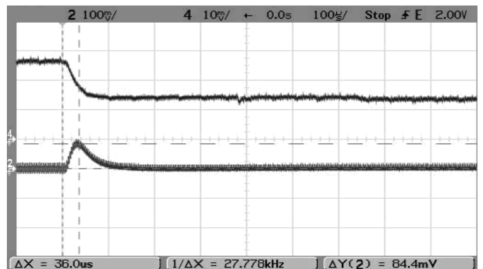
Step Load Transient Response (Vin=5V, Vout=1.2V, Cload=0, Iout=5A to 2.5A) Trace 2=Vout, 100 mV/div. Trace 4=Iout, 2A/div.
