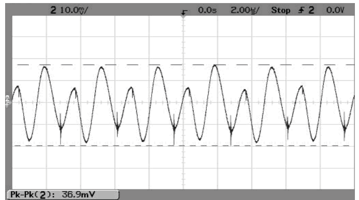
Output Ripple and Noise (Vin=5V, Vout=1.2V, Iout=5A, Cload=0, ScopeBW=100MHz)
