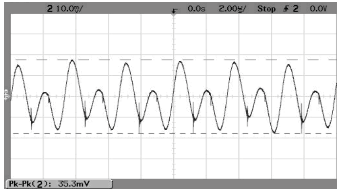
Output Ripple and Noise (Vin=5V, Vout=1.5V, Iout=5A, Cload=0, ScopeBW=100MHz)
