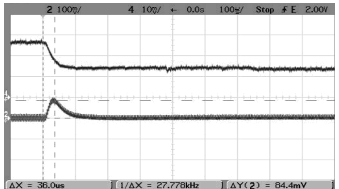
Step Load Transient Response (Vin=5V, Vout=1.5V, Cload=0, Iout=5A to 2.5A) Trace 2=Vout, 100 mV/div. Trace 4=Iout, 2A/div.
