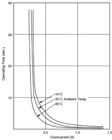
Operating Time (Typical Curve)
