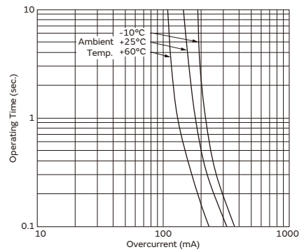
PRG18BC6R8MM1RB
