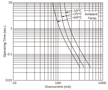
PRG18BC150MM1RB
