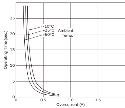
PTGL07AR820M9A51B0
