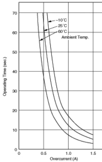
Operating Time (Typical Curve)
