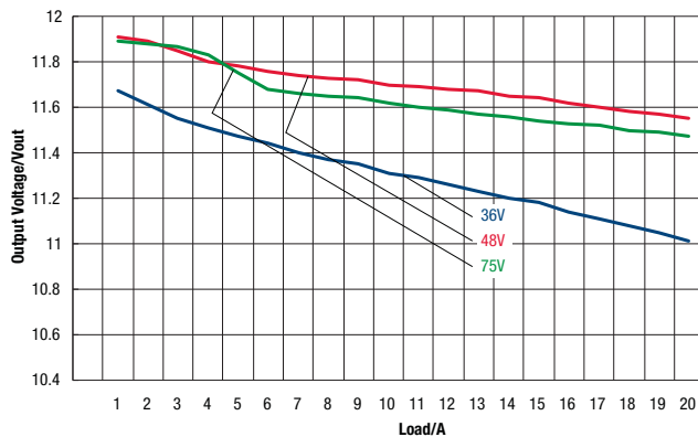
Typical Output Voltage (Vout) Vs. Output load at +25°C
