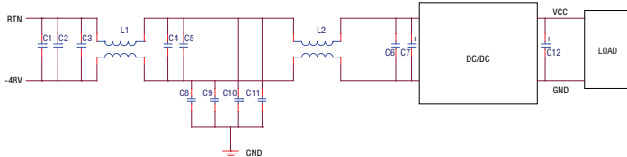
Figure 8. Conducted Emissions Test Circuit
